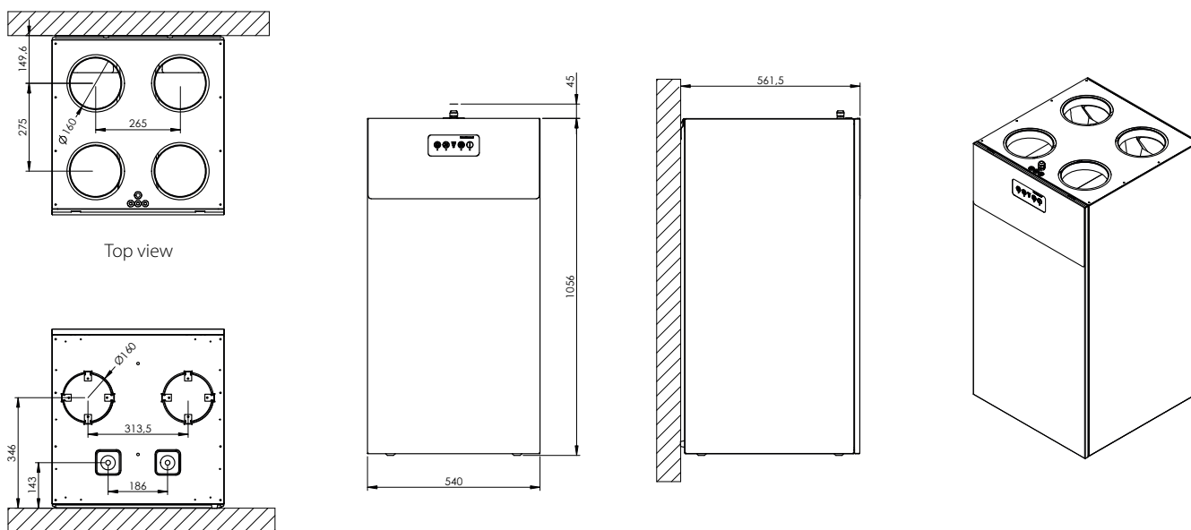
Top view
